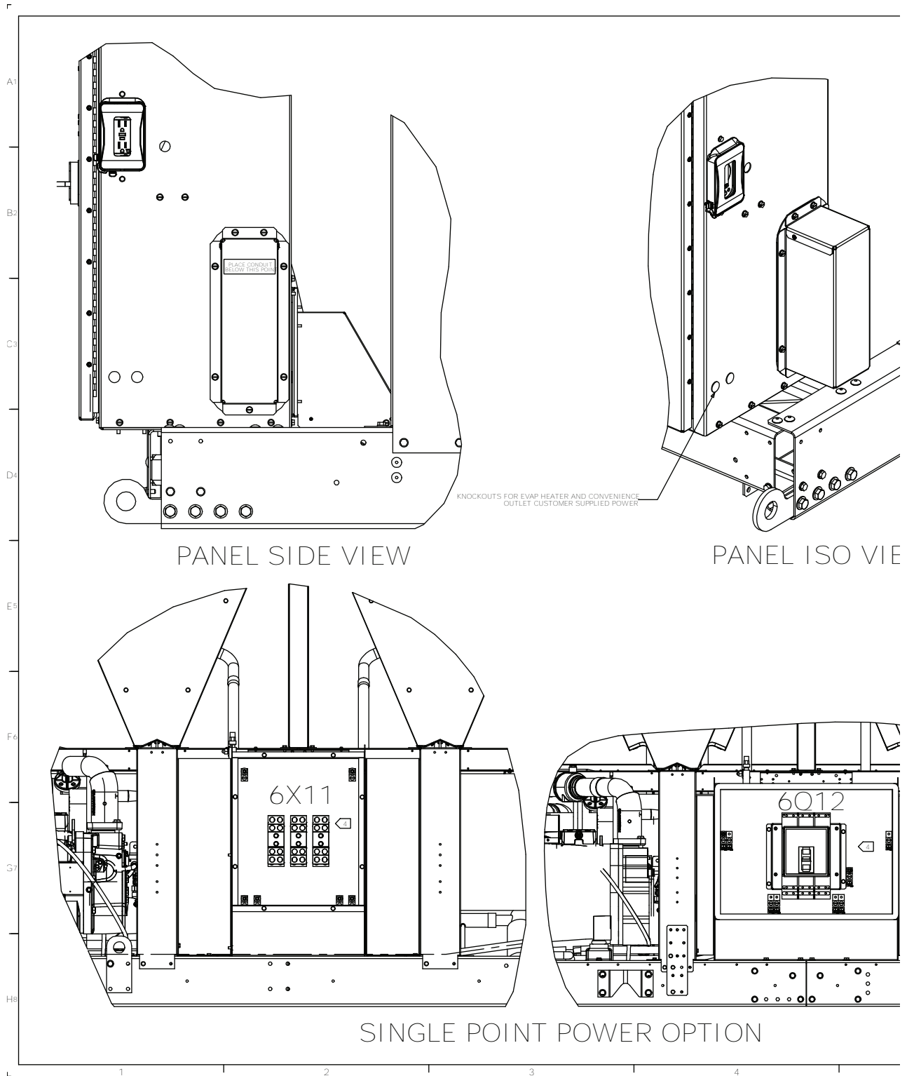
Figure 12. Field wiring, 280 to 520 ton, sheet 2
