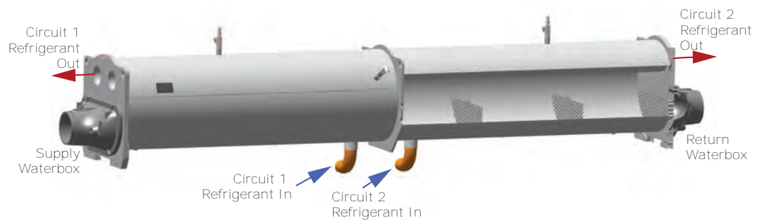
Figure 3. CHIL evaporator, 280 to 520 tons, 1-pass
