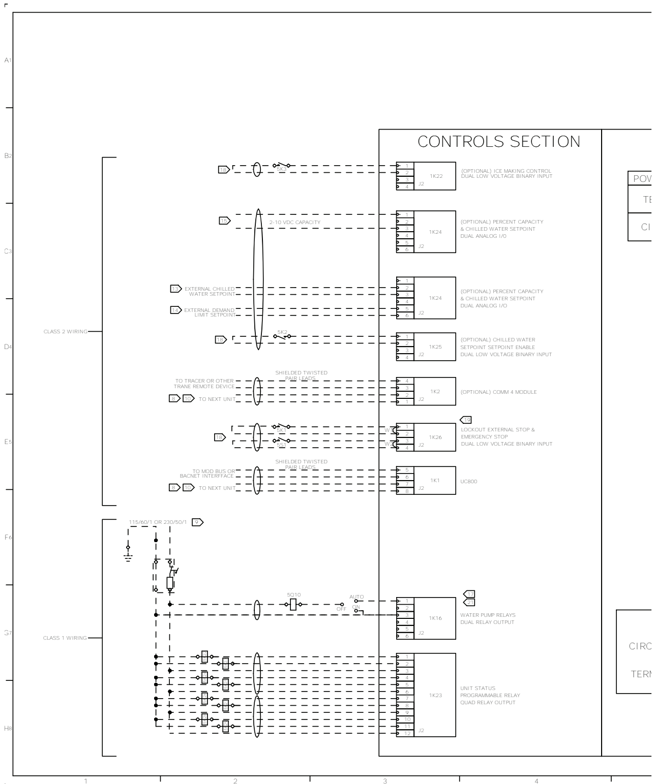
Figure 9. Field wiring, 115 to 270 ton, sheet 1
