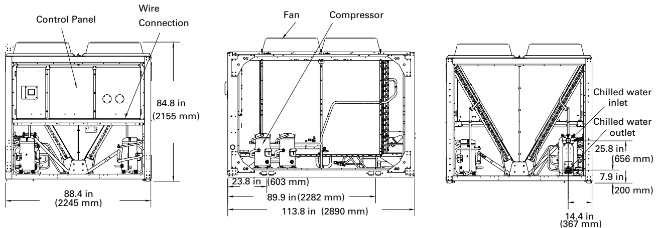
Figure 8. CGAM 40 and 52 ton
