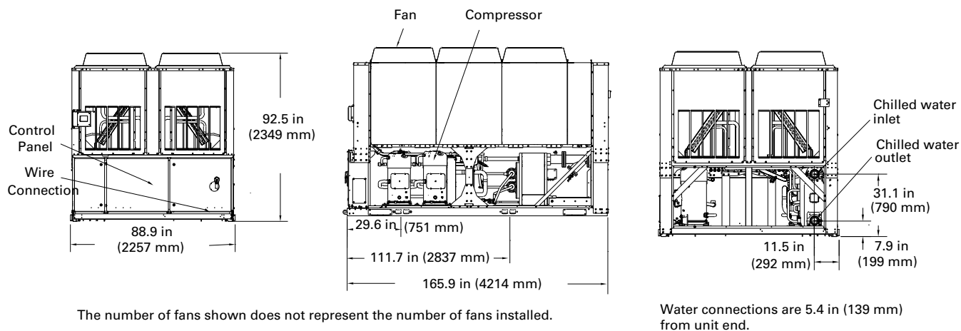
Figure 14. CGAM 100, 110 and 120 ton
