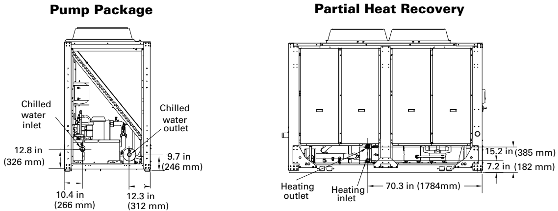
Figure 18. CGAM 20 and 26 ton - pump package, partial heat recovery unit water connections
