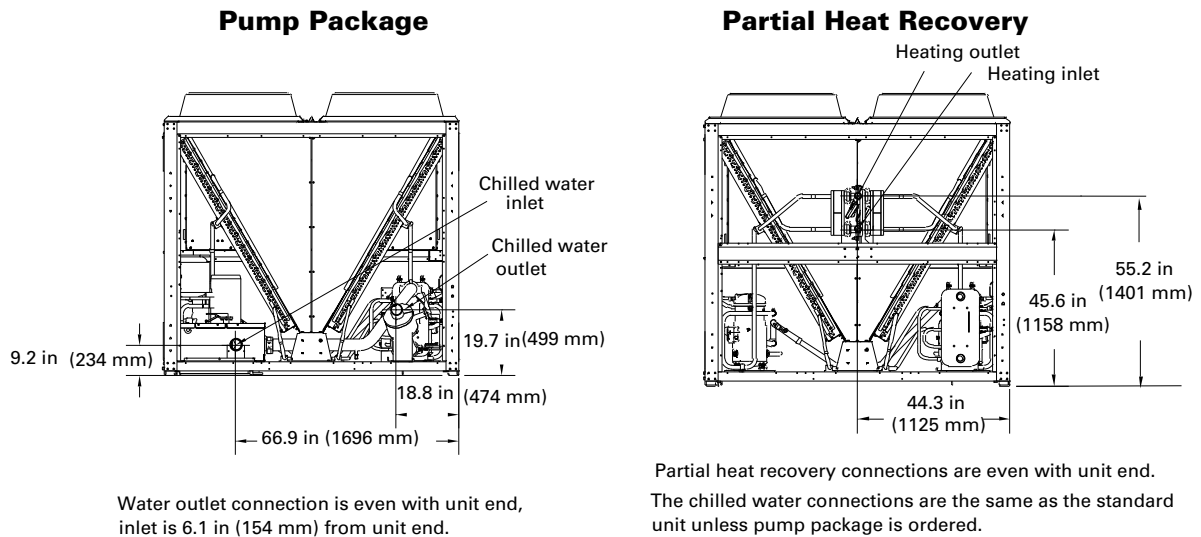
Figure 21. CGAM60 and 70 ton- pump package, partial heat recovery unit water connections
