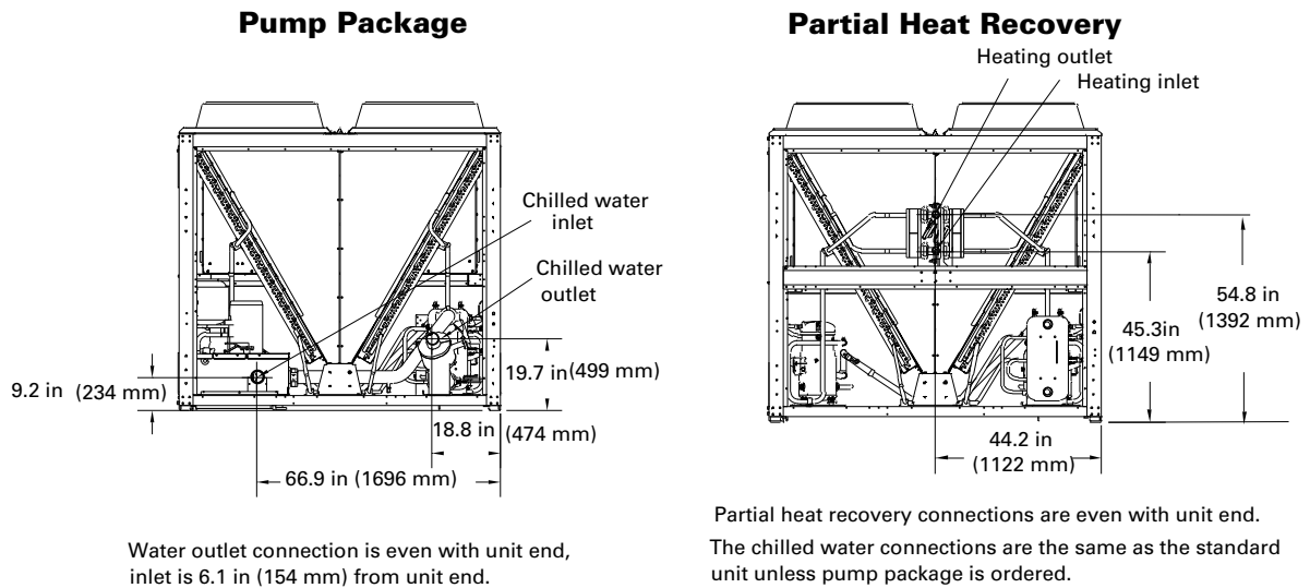
Figure 20. CGAM 40 and 52 ton- pump package, partial heat recovery unit water connections
