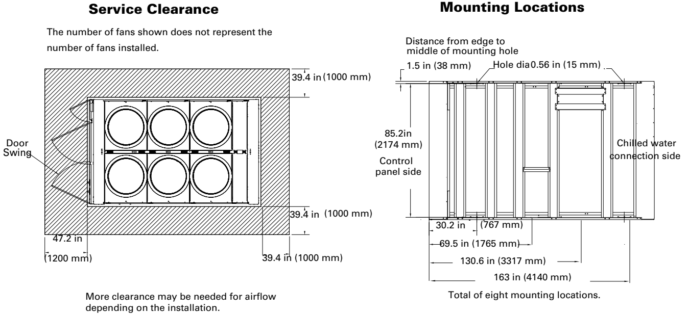
Figure 17. CGAM 130 ton- service clearances and mounting locations
