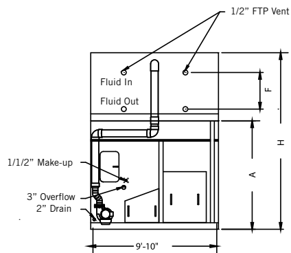
End Elevation: Models Models VF1-1012, 1018, 1024, 1036
