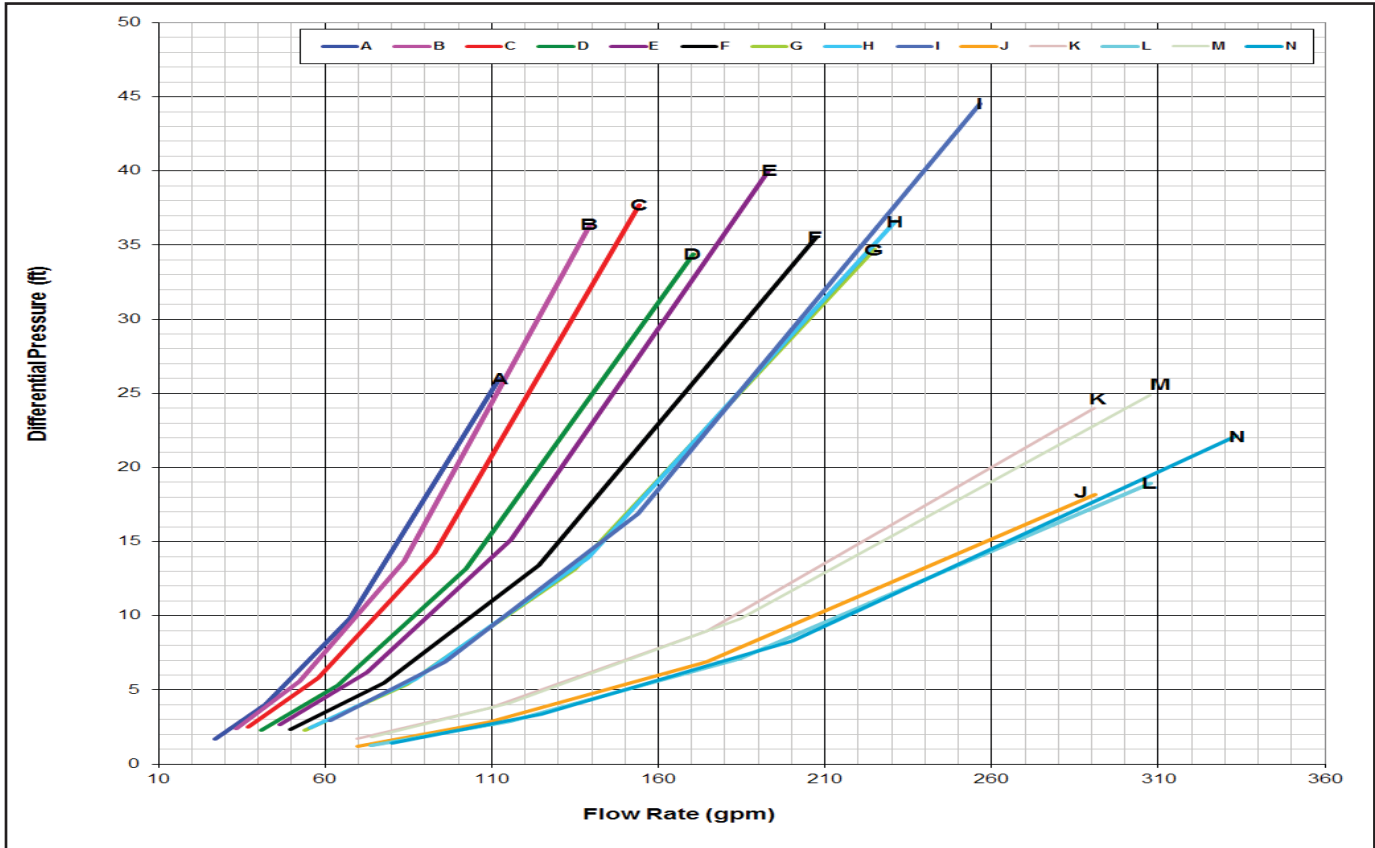
Figure 30: Pressure Drop Curves - Unit Evaporator - AGZ030-AGZ090E (Reference Table 14 on page 23)
