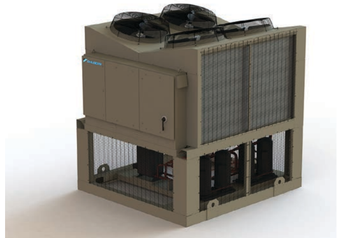
Figure 53: Unit with Base Guards
