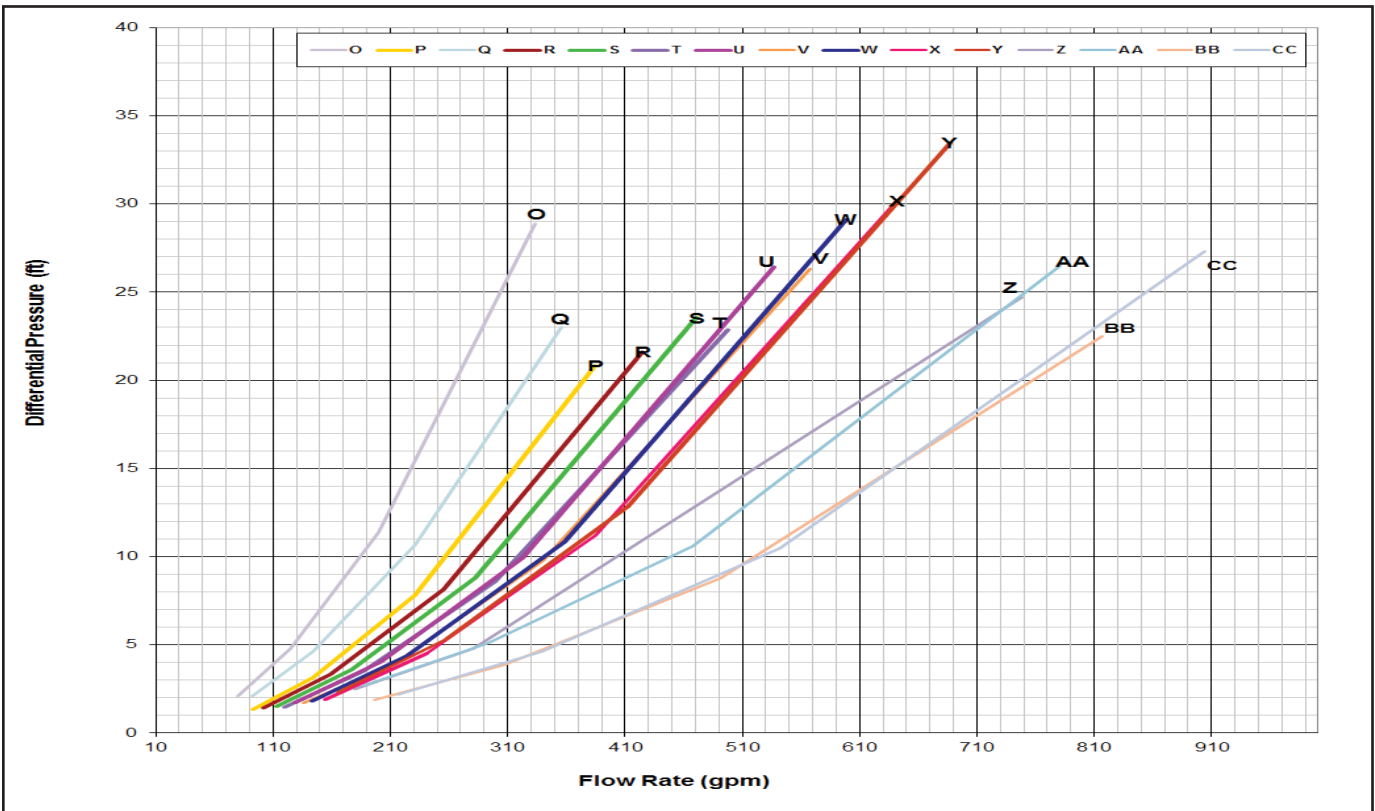
Figure 31: Pressure Drop Curves - Unit Evaporator - AGZ091-AGZ-241E (Reference Table 14 on page 23)
