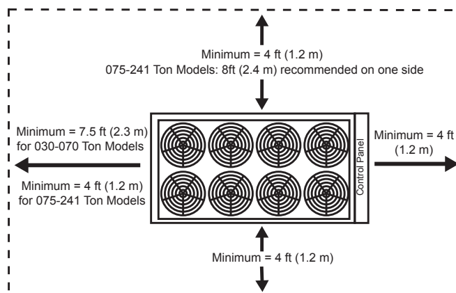
Figure 5: Service Clearance
