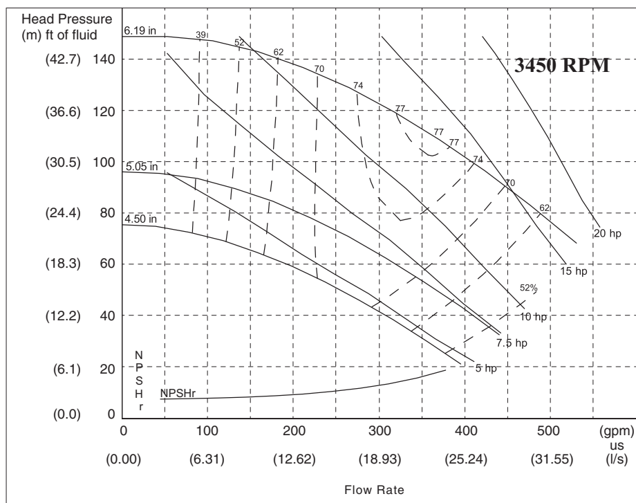
PUMP CURVE VIIB FOR HYDRONIC PACKAGE DUAL PUMP (FRESH WATER)
