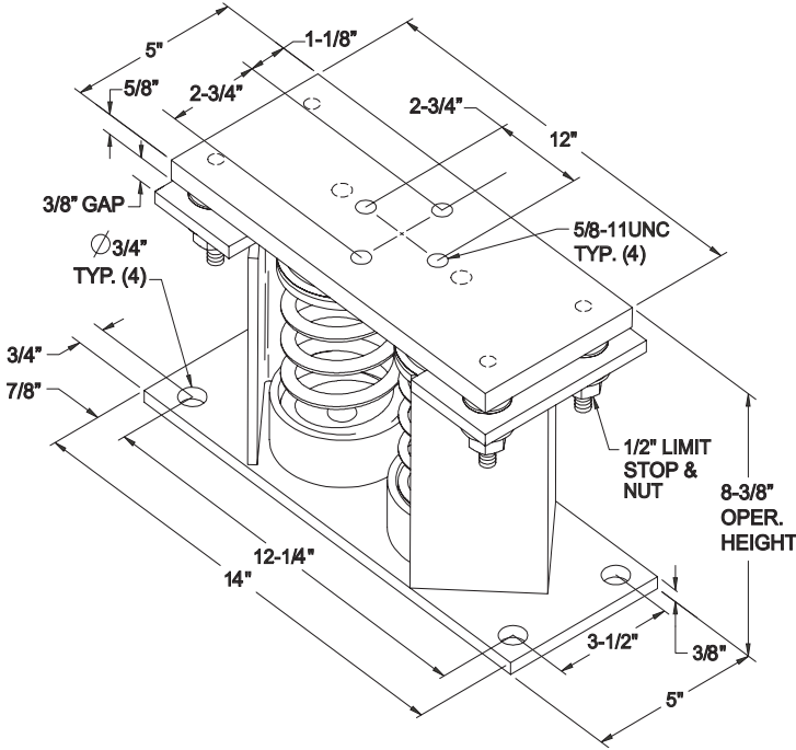
MODEL Y2RSI-2D RESTRAINED VIBRATION ISOLATOR FOR 2\"/>
